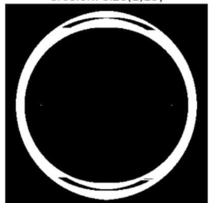
erosion: size(1,15)
